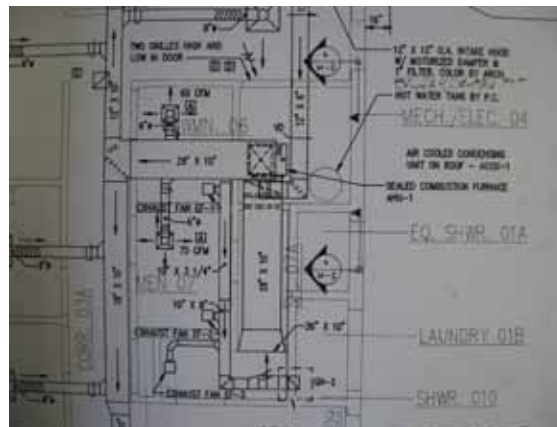
Figure 5-1 – Mechanical plans.
