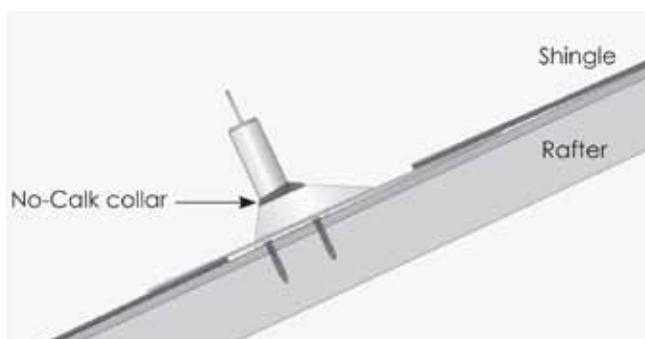
Figure 8-15 — Flashing detail for a cylindrical standoff with boot flashing. (Courtesy of Unirac)
