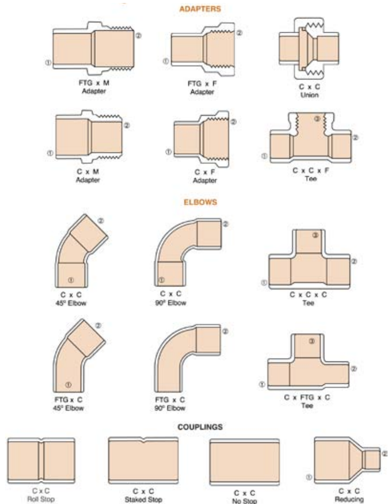
Figure 5-8 — Standard copper fittings with their designated notations.
