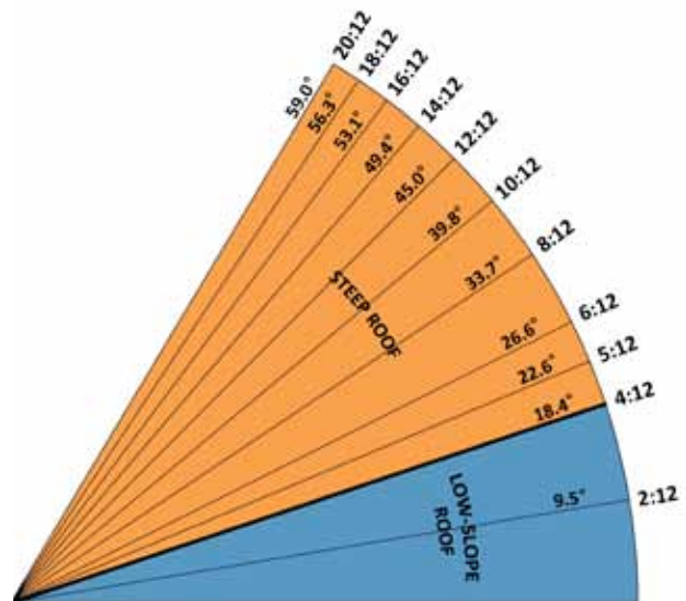
Figure 5-5 – Common roof slopes.
