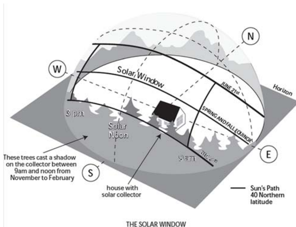
Figure 3-7 — Illustration of the solar window. The top and bottom of the window are defined by the solstices; the edges of the window are defined by a 6-hour span centered on solar noon. (Courtesy of Solar Energy International — www.solarenergy.org )
