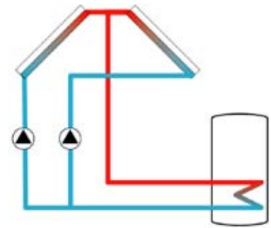
Figure 8-28 — Balancing flow through collector banks through the use of controls. (Courtesy of Resol)
