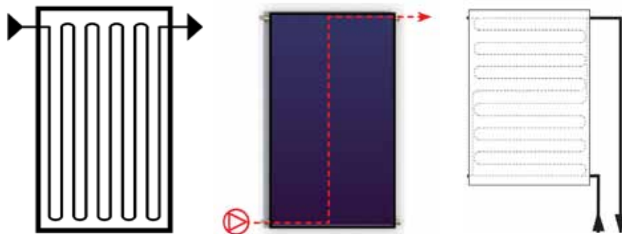
Figure 8-20 — Flow path through various styles of flat plate collectors. (Courtesy of Schüco, Heliodyne, Bosch Thermotechnology)
