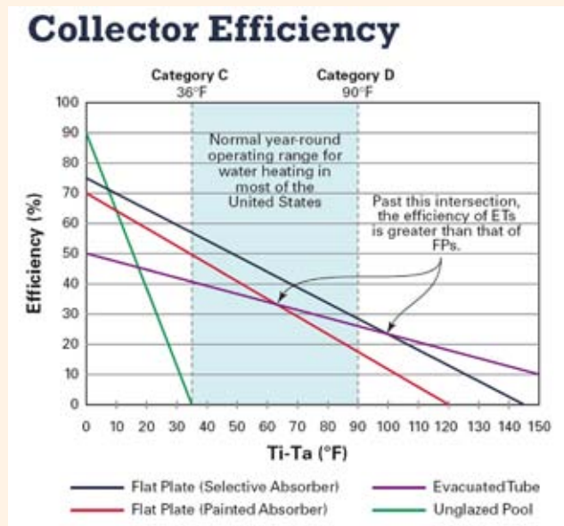
Figure 4-8 — Performance slopes for typical collector styles. (Courtesy of homepower.com)
