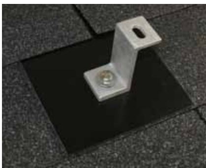
Figure 8-14 — Mechanical flashing for structural attachment points. (Courtesy of EcoFasten Solar)
