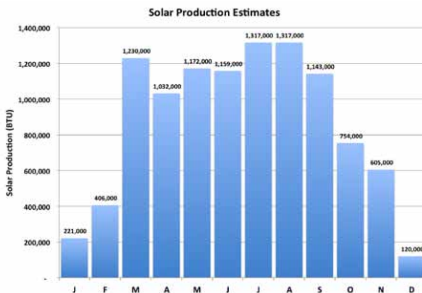
Figure A-2 — Monthly performance estimates for system based on Solar Pathfinder Assistant model
